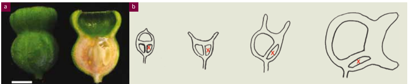
Figure 4 A healthy marri fruit cut at longitudinal section (a) and section diagrams of infected flower bud, flower, immature fruit and mature capsule, showing how the infection of a carpel (indicated by red cross) of a flowering structure can lead to disproportionate growth of the healthy carpels, resulting in the 'horizontal' growth habit (b) (Bar = 10mm).
